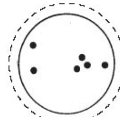
TAURUS, the Bull
