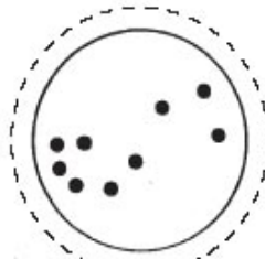
SCORPIUS, the Scorpion
