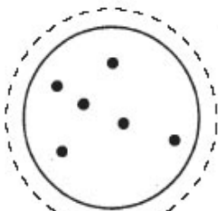
CYGNUS, the Swan
