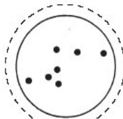
CANIS MAJOR, the Big Dog
