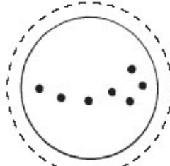
URSA MINOR, the Little Bear
