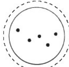
CASSIOPEIA, the Queen
