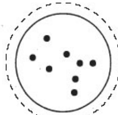
GEMINI, the Twins
