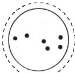
URSA MAJOR, the Great Bear
