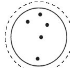
BOOTES, the Herdsman
