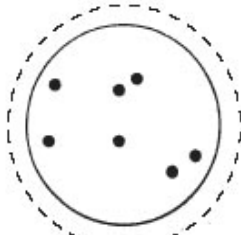
PEGASUS, the Flying Horse
