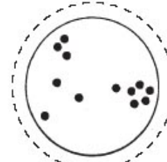
PISCES, the Fishes
